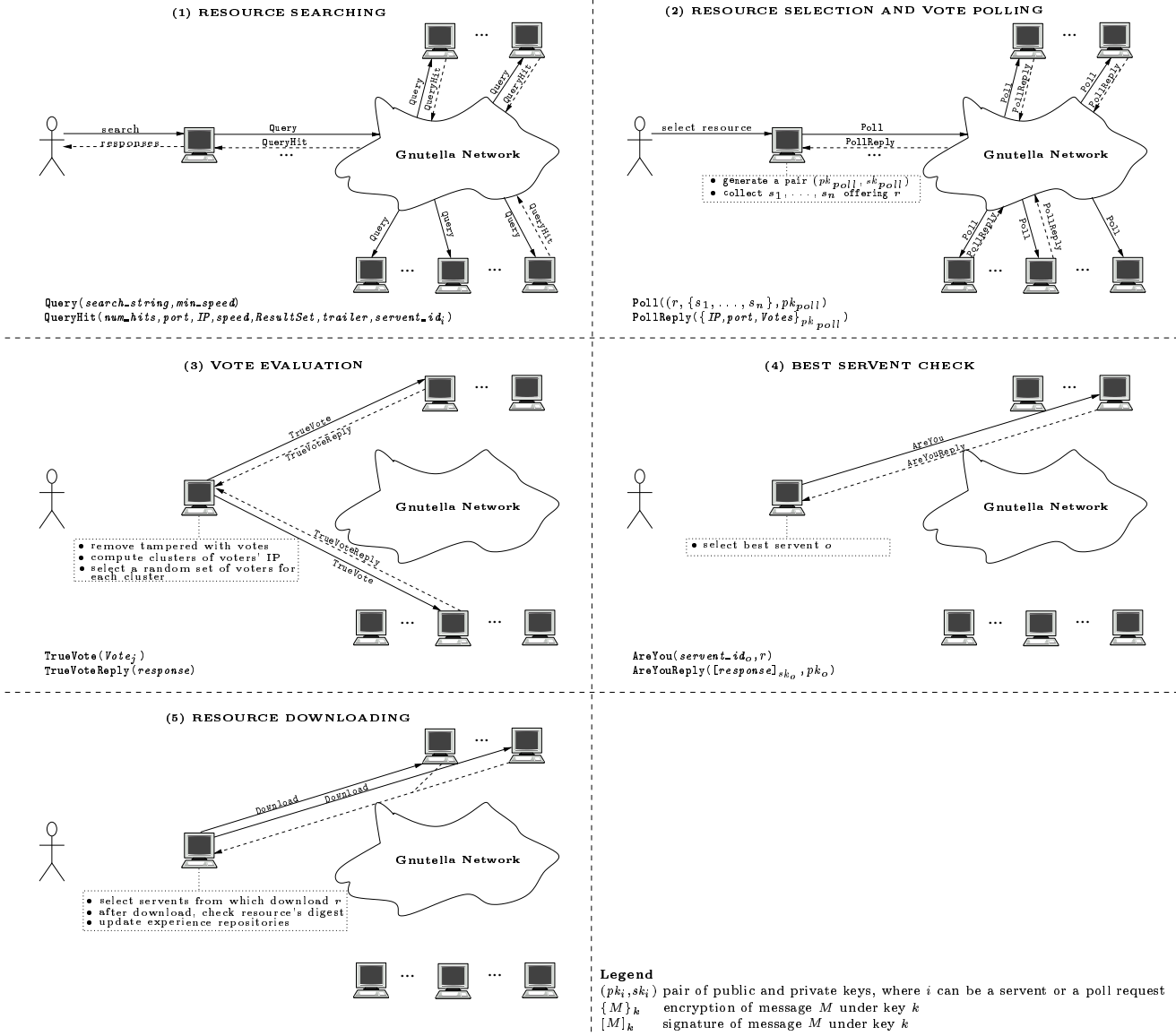
Figure 1: Sequence of messages and operations in the XRep protocol
